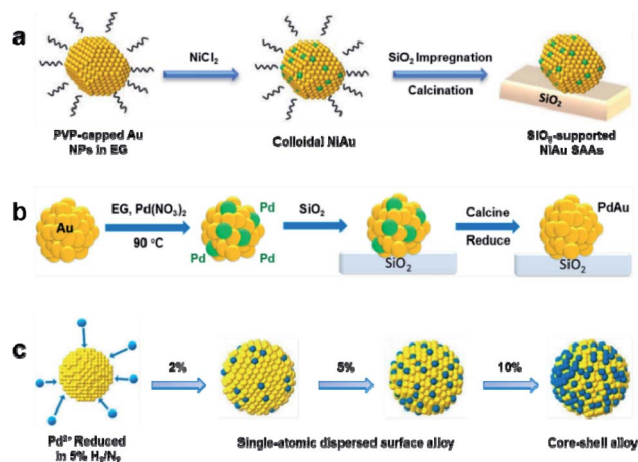
Fig. 5 Sequential reduction method: (a) schematic representation of the sequential reduction method for the synthesis of \text{SiO}_2 -supported NiAu SAAs. Reproduced from ref. 26 with permission from the American Chemical Society, copyright 2020. (b) Schematic illustration of PdAu SAAs synthesis in which the final reduction step leads to migration of Pd to the interior of the NPs. Reproduced from ref. 63 with permission from the author(s), copyright 2021. (c) Illustration of the synthetic scheme for the Pd@Au SAAs with control over the dose of Pd. Reproduced from ref. 64 with permission from the American Chemical Society, copyright 2019.
