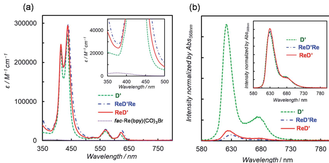
Fig. 3 (a) UV-vis absorption spectra of D' , ReD' , ReD' , and fac -Re(bpy)(CO) 3 Br in DMA. The inset presents the magnification of the near-UV region. (b) Fluorescence spectra of D' , ReD'Re , and ReD' in DMA at 298 K. The inset shows the spectra in toluene. The fluorescence spectra were normalized with the absorbance at the excitation wavelength ( \lambda_{\text{ex}} = 568 nm).
