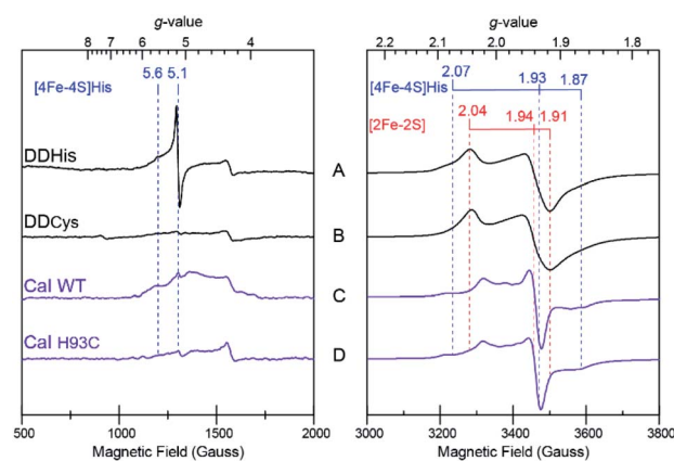
Fig. 4 X-band EPR spectra of distal domain and CaI, with low-field region on left; high-field region, on right. (A) DDHis (230 \mu M ) (B) DDCys (230 \mu M ) (C) CaI WT (200 \mu M ) (D) CaI H93C (200 \mu M ). All samples were prepared under identical conditions and reduced with dithionite in pH 8.8 buffer. Signal assignments for the [4Fe-4S]His and [2Fe-2S] clusters are indicated. Measurement conditions: microwave frequency 9.39 GHz; modulation frequency, 100 kHz; modulation amplitude, 10 Gauss; microwave power, 1 mW (A and B), 10 mW (500–2000 Gauss C and D), 1 mW (3000–4000 Gauss C and D); sample temperature: 10 K.
