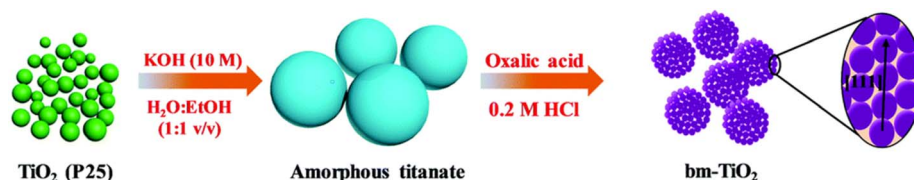
Fig. 3 Preparation process of mesomorphic \text{TiO}_2 with brookite phase. 39
