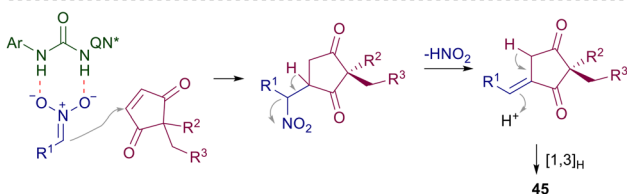
Scheme 33 Alkylation desymmetrization of cyclopentenedione derivatives catalyzed by quinine-derived chiral urea 44 .
