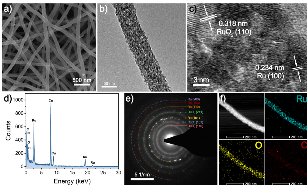
Fig. 1 (a) SEM image, (b) TEM image, (c) HRTEM image, (d) EDX spectrum, (e) SAED pattern, (f) HAADF-STEM micrograph and EDX mappings of synthesized \text{RuO}_2/\text{Ru} -CNFs-350.
