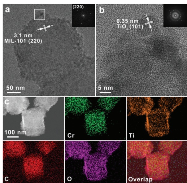
Fig. 2 TEM images of a single MOF@TiO 2 -A core-shell nanoparticle (a) and enlarged high-resolution TEM image of the TiO 2 shell corresponding to the rectangular area in a (b). High-magnification HAADF-STEM image of MOF@TiO 2 -A (c) and the corresponding EDX elemental mapping results. Insets in a and b correspond to the fast Fourier transform (FFT) images of MOF and TiO 2 crystals.
