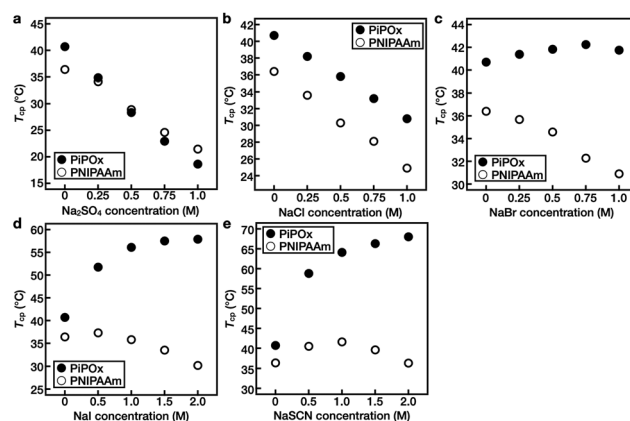
Fig. 4 T_{cp} profiles of PNIPAAm (open circles) and PiPOx (closed circles) in salt solutions as a function of the (a) Na 2 SO 4 , (b) NaCl, (c) NaBr, (d) NaI, and (e) NaSCN concentrations. The concentration of the polymer was 1 wt%.
