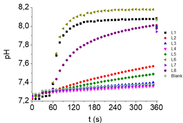
Fig. 4 Variation of pH upon addition of compounds L1–L8 (0.5 \mu\text{M} ) to 7:3 POPC:cholesterol vesicles (0.5 mM POPC). Vesicles (loaded with a 126.2 mM \text{NaNO}_3 solution buffered to pH 7.2 with 10 mM \text{NaH}_2\text{PO}_4 , and containing 1 mM HPTS; ionic strength (I.S.) 150 mM), were suspended in a \text{NaNO}_3 solution (126.2 mM \text{NaNO}_3 buffered to pH 7.2 with 10 mM \text{NaH}_2\text{PO}_4 ; I.S. 150 mM). At t = 30 s an aliquot of a NaOH solution (12.5 \mu\text{L} , 0.5 M) was added, and at t = 60 s the anion carrier was added. The blank is DMSO (1.25 \mu\text{L} ). Each trace represents the average of at least three trials, performed with three batches of vesicles.
