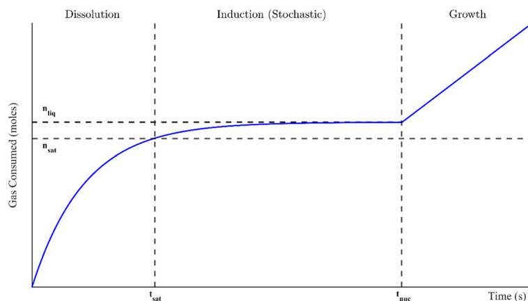
Fig. 1 Schematic of a typical hydrate formation profile through guest gas consumption. Here, n_{sat} is the molar saturation value that occurs at t_{sat} and n_{liq} is the final number of moles in the supersaturated solution at nucleation, which occurs at t_{nuc} .
