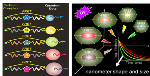
Fig. 12 Principle of multiplexed Tb-complex to QDs FRET applied for ultra-sensitive diagnostics (left) and spectroscopic ruler measurements (right). Reprinted with permission from ref. 207 and 208. Copyright (2010), Wiley-VCH Verlag GmbH & Co. KGaA.
