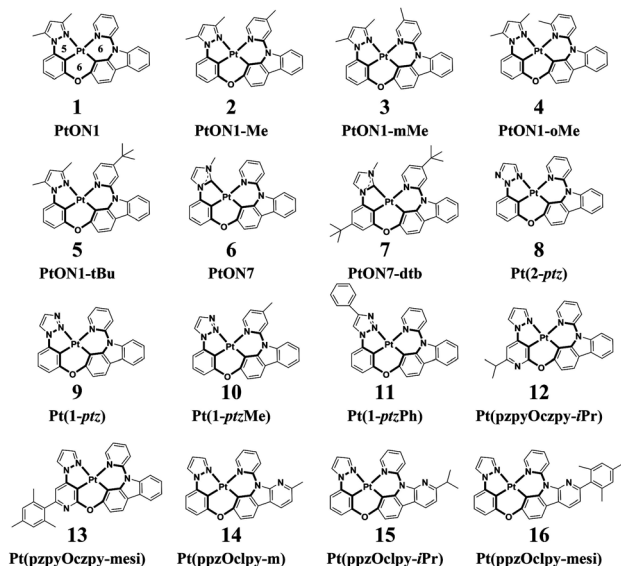
Scheme 1 Structures of 16 blue-emitting tetradentate Pt(II) emitters containing fused 5/6/6 metalocycles. ( 2-ptz = 2-phenyl-1,2,3-triazole; 1-ptz = 1-phenyl-1,2,3-triazole; ppz = phenyl-pyrazol; ppzy = pyrazol-pyridine; czpy = pyridyl-carbazole; clpy = pyridyl-carboline; iPr = iso propyl; mes = mesityl)
