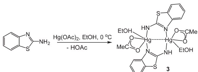
Scheme 2 Formation of \mathbf{3} from reaction of abt and \text{Hg}(\text{OAc})_2 at 0 °C.
