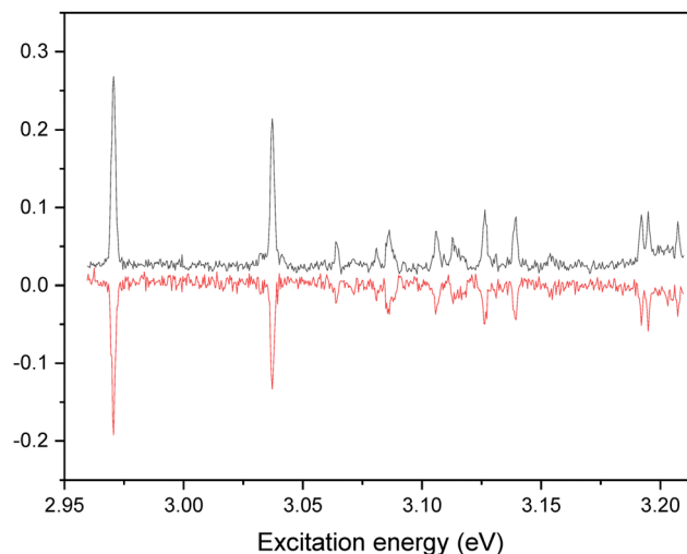
Fig. 4 IR-UV dip signal of C^+ with the IR wavelength set at 3350\text{ cm}^{-1} compared to the vibronic spectrum recorded in the 2.95–3.22 eV.
