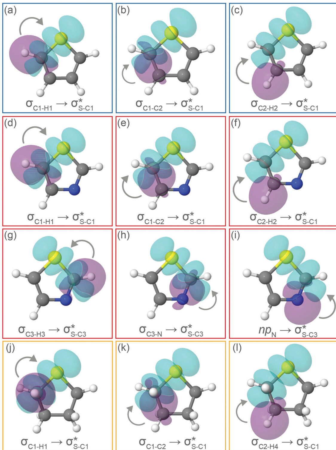
Fig. 5 Natural Bond Orbitals representation of the Second-Order Perturbation interaction between donor (in purple) and \sigma_{\text{S-C}}^* acceptor (in cyan) for (a–c) thiophene, (d–i) thiazole, and (j–l) twisted thiolane conformer in the electronic ground state.
