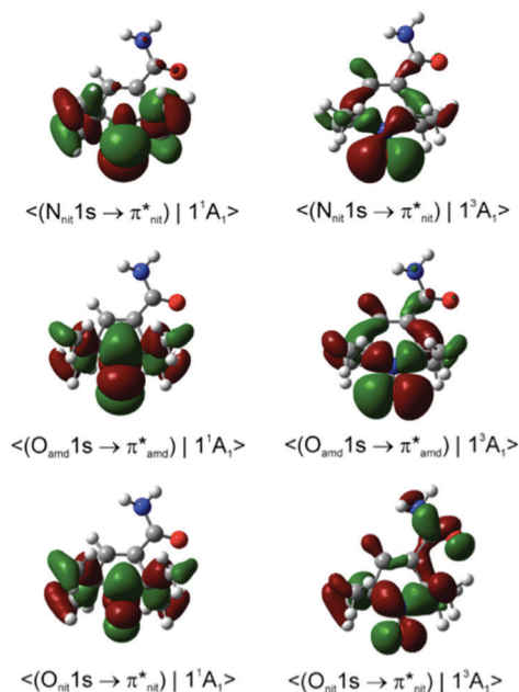
Fig. 8 Dyson spin orbitals of nit9 at the CAM-B3LYP//mixed level. The initial core-to-valence states concern the excitation from the 1s orbitals of amide (amd) or nitroxy (nit) N or O atoms. The final states are the lowest singlet and triplet nit9 cations ( 1^1A_1 and 1^3A_1 ).
