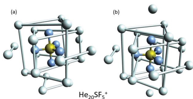
Fig. 7 Selected geometries corresponding to \text{He}_{20} \text{SF}_5^+ . (a) Minimum energy configuration as predicted by EA optimizations and (b) a closed symmetric structure of about 7 meV above the minimum shown in panel (a). As in Fig. 6, He atoms have been artificially bonded as a guide to the eye to distinguish structures around the dopant.
