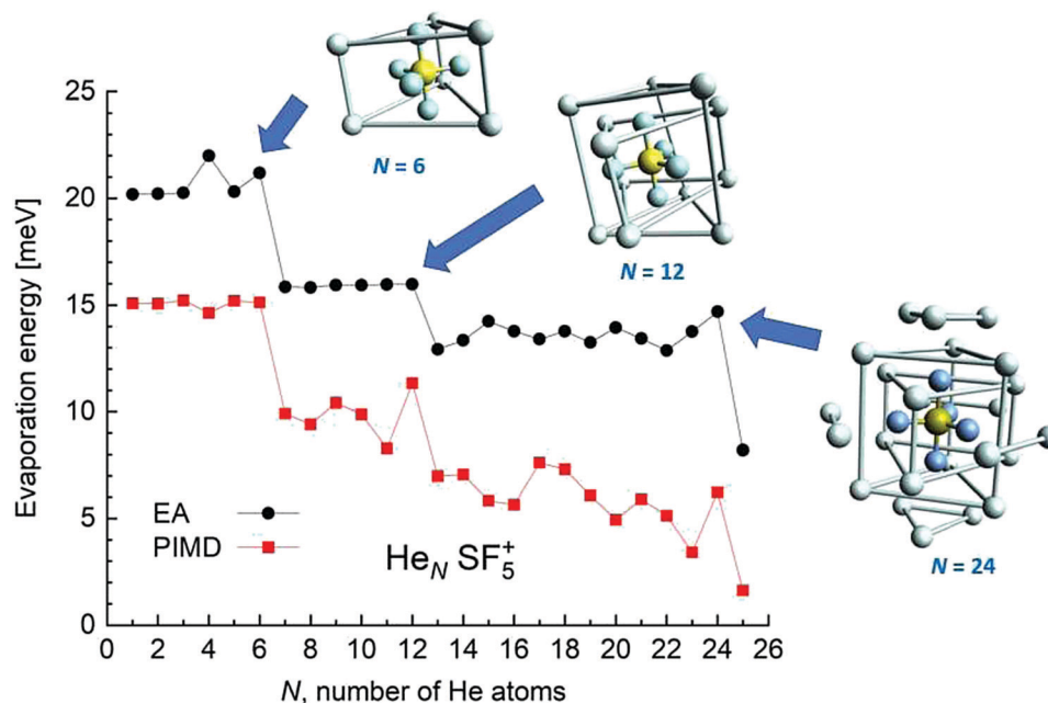
Fig. 6 Evaporation energies \Delta E_N for the \text{He}_N \text{SF}_5^+ clusters calculated using the EA (black circles) and PIMD (red squares) methods as a function of the number of He atoms, N . The figure includes the minimum energy structures observed using the classical EA approach for N = 6, 12 and 24 cases. Bonds between some He atoms have been artificially added in order to illustrate the successive helium structures around the dopant.
