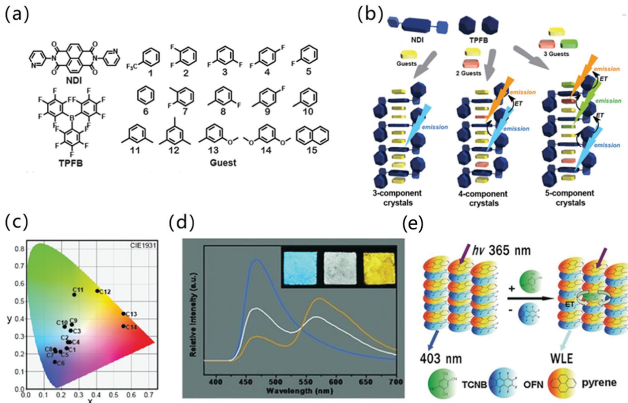
Fig. 6 (a) The structure of NDI, TPFB and aromatic guests composed of three, four, and five-component cococrystals. (b) Schematic illustration of three-, four-, and five-component crystalline materials. (c) Emission colors in the CIE 1931 chromaticity diagram of multi-component cococrystals. Reprinted with permission from ref. 46. Copyright 2019. The Royal Society of Chemistry. (d) Steady state emission spectra of mixed CT complex microtube films spin-coated on a quartz substrate at doping concentrations of 0 (blue), 0.015% (white), and 0.1% (orange) upon excitation with 365 nm. Insets show the corresponding photographs excited with a UV lamp (365 nm). The excitation wavelength is 365 nm. Reprinted with permission from ref. 48. Copyright © 2012 Wiley-VCH Verlag GmbH & Co. KGaA, Weinheim. (e) The energy transfer mechanism of pyrene-OFN and pyrene-TCNB. Reprinted with permission from ref. 49. Copyright © 2017 Wiley-VCH Verlag GmbH & Co. KGaA, Weinheim.
