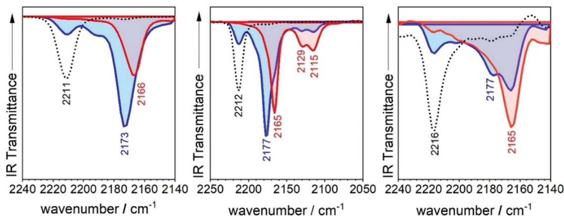
Fig. 5 Infrared spectra taken during the spectroelectrochemical reduction in 0.1 M TBPFe in \text{CH}_2\text{Cl}_2 at room temperature of 3TQ (left), B-3TQ (middle) and B3-3TQ (right). Neutral (broken lines), radical anions (blue shaded) and dianions (red shaded).
