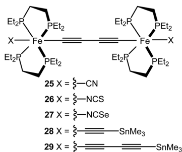
Fig. 11 Structures of 25–29.
