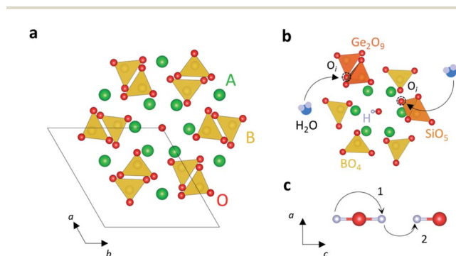
Fig. 12 (a) Crystal structure of apatite \text{A}_{10-x}\text{B}_6\text{O}_{26\pm\delta} . (b) Representation of the water absorption mechanism. The interstitial \text{O}_i site is close to the centre of the La channel in Si-apatites, and hydration leads to the formation of distorted \text{SiO}_5 units. In the Ge-apatite the interstitial site is in proximity of the \text{GeO}_4 tetrahedra, with the water absorption resulting in the creation of \text{Ge}_2\text{O}_9 units. Protons are located on the oxide ion at the centre of the La ring. (c) Schematic of the possible proton transfer mechanism composed by rotation (1) and hopping (2) within the channel parallel to the c -axis.
