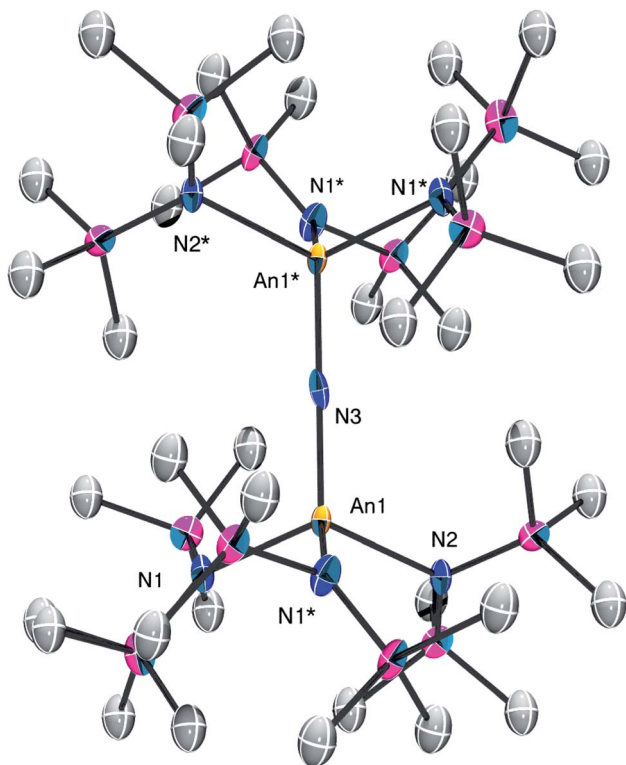
Fig. 1 Solid-state molecular structure of 2 shown with 50% probability ellipsoids. [K(18-crown-6)(THF) 2 ] + counterion and hydrogen atoms are removed for clarity.
