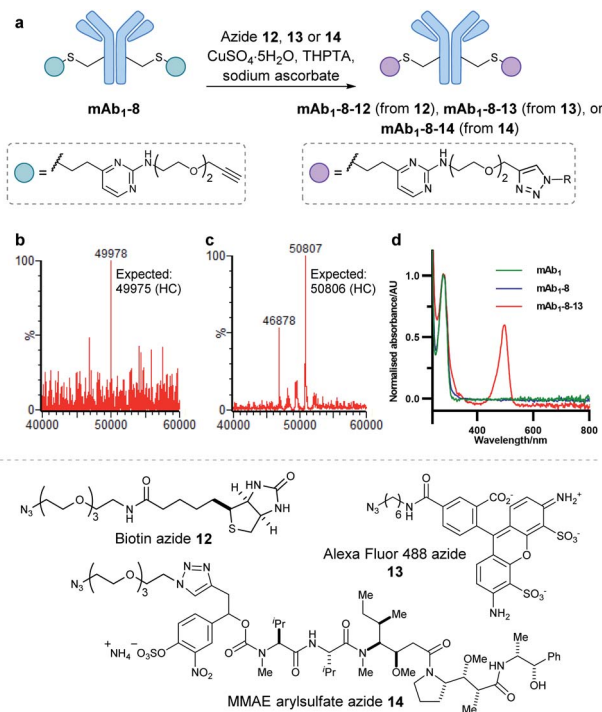
Fig. 5 (a) On-protein copper catalysed azide-alkyne cycloaddition (CuAAC) reactions to functionalise alkyne antibody mAb 1 -8 . This antibody was successfully modified with biotin 12 , Alexa Fluor 488 fluorophore 13 and arylsulfate-MMAE 14 . (b) Deconvoluted mass spectrum of mAb 1 -8-12 heavy chain. (c) Deconvoluted mass spectrum of mAb 1 -8-14 heavy chain. Species with 46 878 Da correspond to light chain dimer. (d) UV-vis spectrum of unmodified mAb 1 , mAb 1 -8 , and mAb 1 -8-13 . Bioconjugate mAb 1 -8-13 displayed a fluorophore-to-antibody ratio of 1.9.
