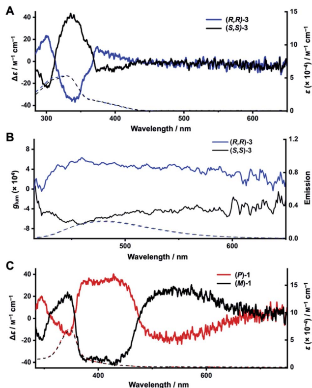
Fig. 5 Chiroptical properties of diketeto[6]CPPs and DBP[6]CPPs ( 5 \times 10^{-5} M in toluene, 20 °C). (A) ECD (solid lines) and UV/Vis absorption spectra (dotted lines) of (R,R) - and (S,S) -3; (B) CPL (solid lines) and fluorescence (dotted lines) spectra of (R,R) - and (S,S) -3; (C) ECD (solid lines) and UV/Vis absorption spectra (dotted lines) of (P) - and (M) -1.
