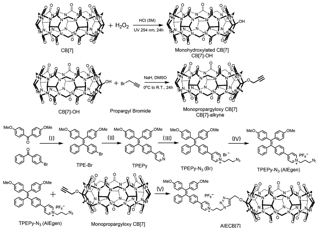
Scheme 2 The Synthetic route for AIECB[7]. Reagents and conditions: (I) \text{TiCl}_4 , Zn dust, anhydrous THF, -78\text{ }^\circ\text{C} , and 24 h; (II) 4-pyridinylboronic acid, \text{Pd}(\text{PPh}_3)_4 , TBAB, 2\text{M K}_2\text{CO}_3 (aq), THF, 80\text{ }^\circ\text{C} , and 5 h; (III) 1-azido-3-bromopropane, DMF, 100\text{ }^\circ\text{C} , and 12 h; (IV) \text{KPF}_6 ; (V) \text{CuSO}_4 , sodium ascorbate, DMSO, 80\text{ }^\circ\text{C} , and 24 h.
