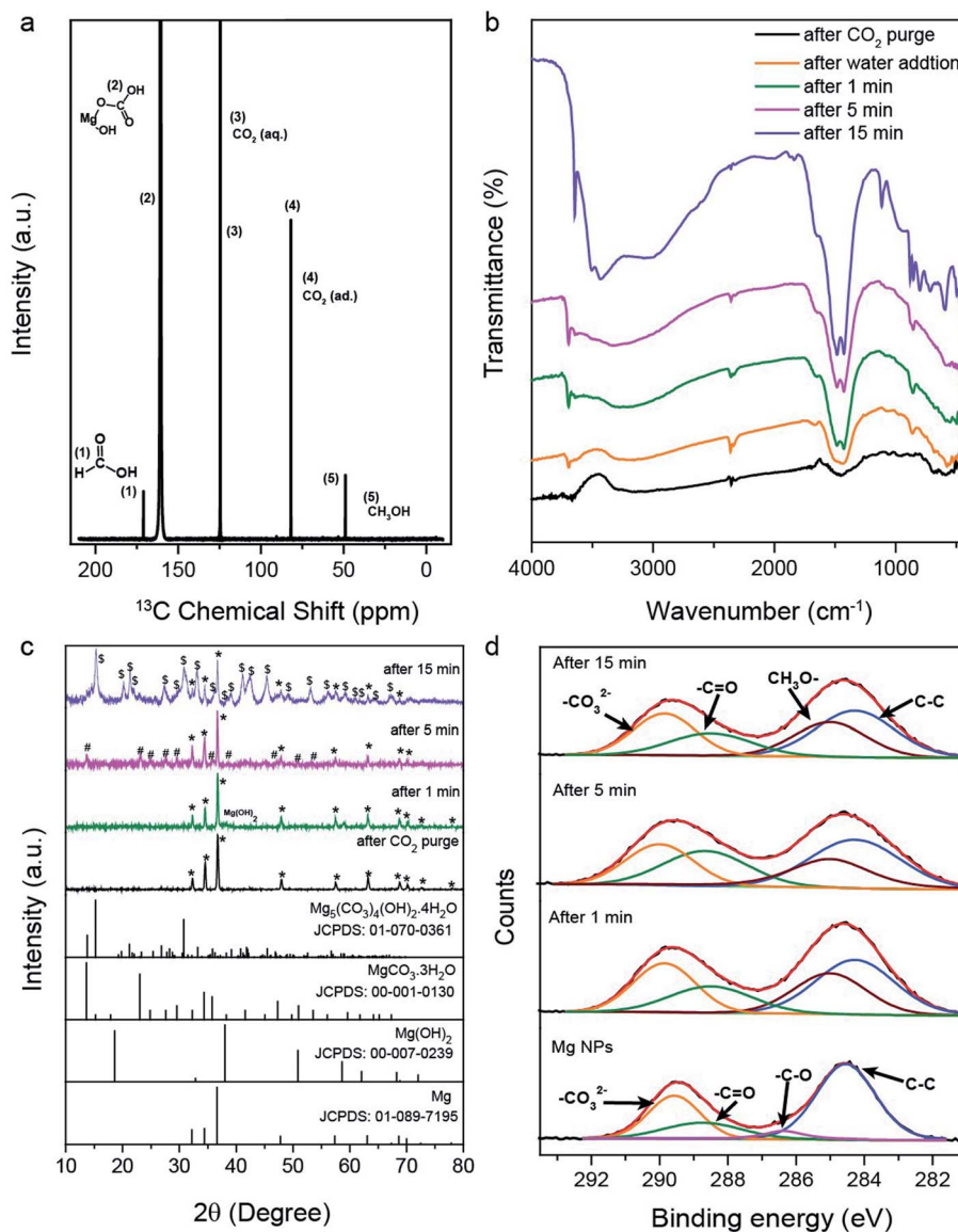
Fig. 2 (a) ^{13}\text{C} NMR spectrum of the reaction mixture (using labeled ^{13}\text{C} ) after 1 h of reaction on Mg NPs; (b) FTIR spectra, (c) PXRD patterns and (d) XPS C 1s spectra of solid products recovered after 1, 5, and 15 min of the reaction of \text{CO}_2 with Mg NPs and water, at room temperature and atmospheric pressure. (*Mg metal, # \text{MgCO}_3 \cdot 3\text{H}_2\text{O} and ^{\text{S}}\text{Mg}_5(\text{CO}_3)_4(\text{OH})_2 \cdot 4\text{H}_2\text{O} ). Standard XRD patterns of Mg (JCPDS no.: 01-089-7195), \text{Mg}(\text{OH})_2 (JCPDS no.: 00-007-0239), \text{MgCO}_3 \cdot 3\text{H}_2\text{O} (JCPDS no.: 00-001-0130) and \text{Mg}_5(\text{CO}_3)_4(\text{OH})_2 \cdot 4\text{H}_2\text{O} (JCPDS no.: 01-070-0361) are included in (c). In (d), orange -\text{CO}_3^{2-} , green -\text{C}=\text{O} , violet -\text{C}-\text{O} , blue -\text{C}-\text{C} , and purple -\text{CH}_3-\text{O} .
