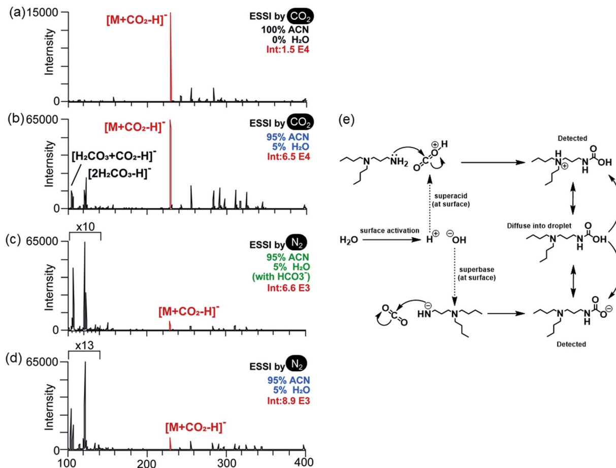
Fig. 4 Droplet reaction showing negative ion ESI mass spectra of (a) ACN droplets and (b) 5% water in ACN droplets with interfacial \text{CO}_2 (c) 5% water in ACN droplets bicarbonate (added) and (d) droplet reaction of 5% water in ACN droplets with room \text{CO}_2 . Autoionization at the charged interface gives superbase which deprotonates the amine, allowing reaction with \text{CO}_2 to form the carbamate anion. (e) Mechanism of superacid/superbase assisted carbamic acid formation at the droplet interface. Small amounts of water present in the droplet generate superacid/superbase at the interface in the presence of a high field, and subsequently activate the carbon dioxide/amine by protonating the carbon dioxide/deprotonating the amine. Note that the species proposed here are the ionic species at the reacting functional groups.
