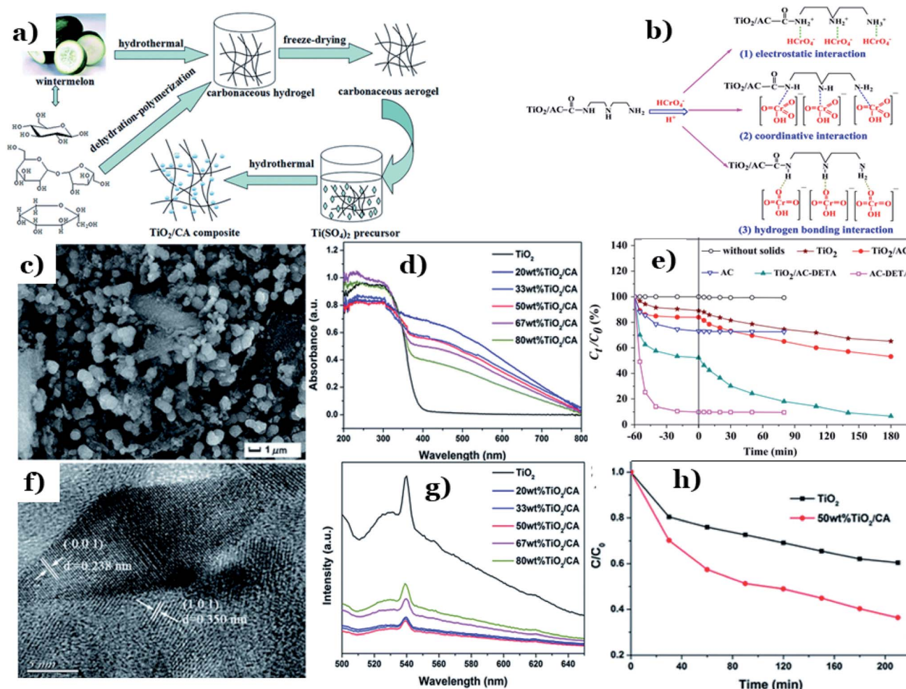
Fig. 9 The synthetic pathway to a TiO 2 /CA composite (a); SEM (c) and HRTEM (f) images of the 50 wt% TiO 2 /CA composite; UV-vis DRS spectra of as-prepared samples (d); PL emission spectra of TiO 2 and the TiO 2 /CA composites (g); and the relationship between C 1 /C 0 and the reaction time (t) during the photodegradation of CIP (h). These figures have been reproduced from ref. 113 with permission from the Royal Society of Chemistry, copyright: 2016. Possible linkages between Cr(vi) and TiO 2 /AC-DETA (b) and the adsorption-photoreduction of Cr(vi) on as-prepared catalysts (e). These figures have been reproduced from ref. 114 with permission from Elsevier, copyright: 2015.
