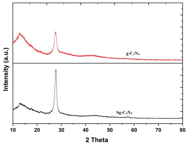
Fig. 2 XRD patterns of g\text{-C}_3\text{N}_4 and \text{Sg-C}_3\text{N}_4 .
