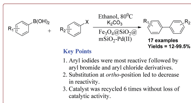
Scheme 8 Suzuki coupling reactions catalyzed by core-shell \text{Fe}_3\text{O}_4@SiO_2@mSiO_2\text{-Pd(II)} nanocatalyst.
