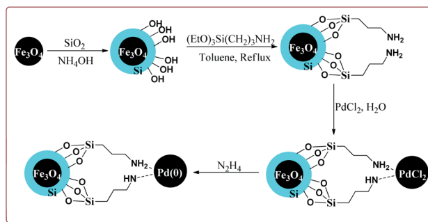
Scheme 11 Synthesis of \text{Fe}_3\text{O}_4@SiO_2 -Pd(0) nanocatalyst.
