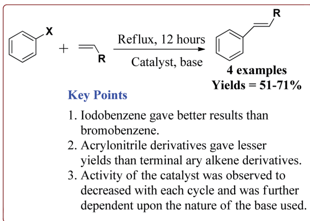
Scheme 15 \text{Pd}/(\text{SiO}_2/\text{Fe}_3\text{O}_4) catalyzed Heck reaction.
