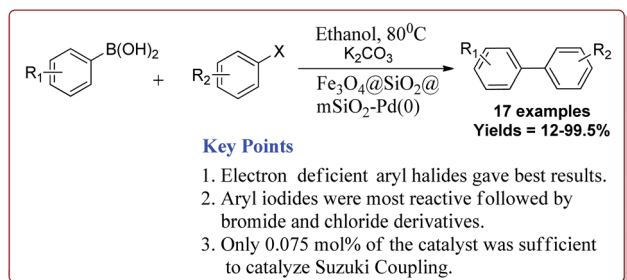
Scheme 10 Suzuki reactions catalyzed by \text{Fe}_3\text{O}_4@SiO_2@mSiO_2 -Pd(0) nanocatalyst.
