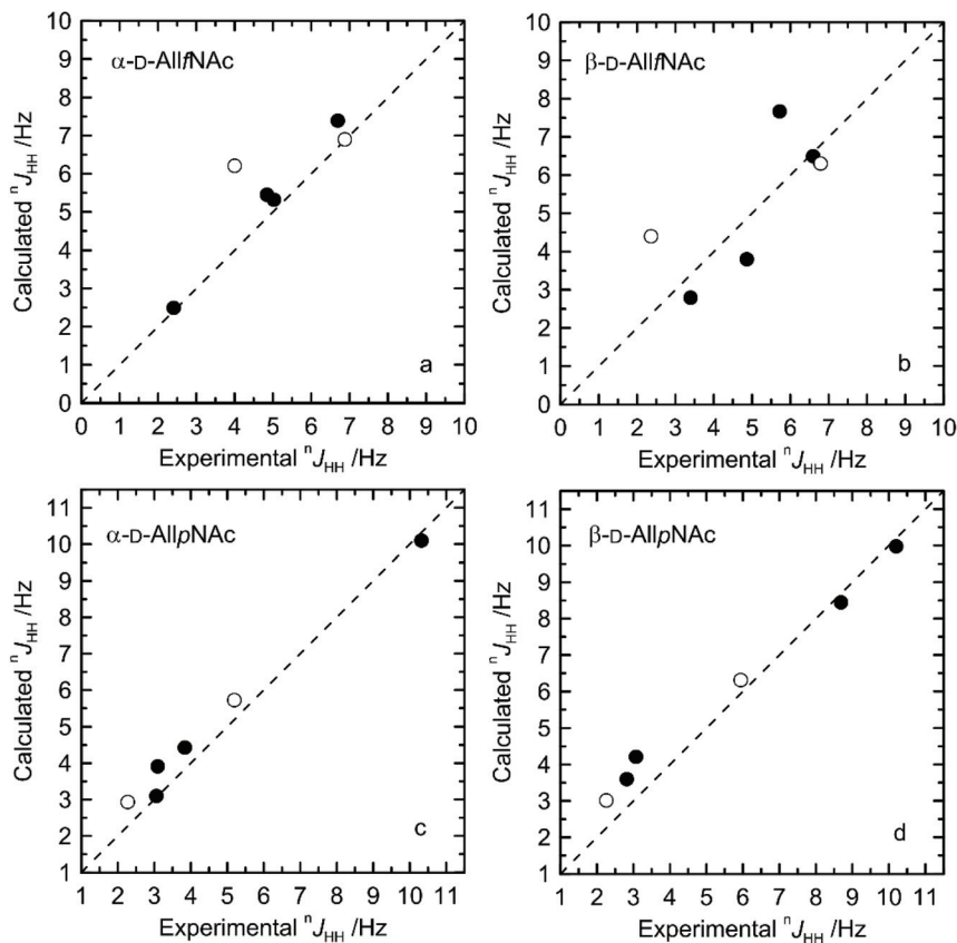
Fig. 4 Calculated vs. experimental {}^nJ_{\text{HH}} presented as absolute values for (a) \alpha\text{-D-AllfNAC} , (b) \beta\text{-D-AllfNAC} , (c) \alpha\text{-D-AllpNAC} and (d) \beta\text{-D-AllpNAC} ; {}^3J_{\text{H5,H6}} are shown by empty circles.
