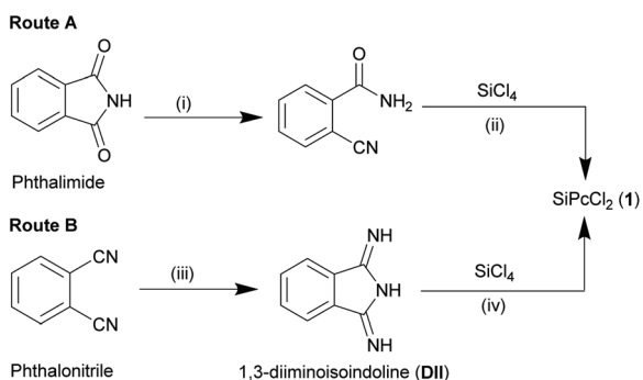
Scheme 2 Synthetic routes for obtaining SiPcCl 2 ( 1 ) starting from precursors phthalimide and phthalonitrile. Reagents and conditions: (i) conc. ammonium hydroxide, 24 h, r.t. (ii) SiCl 4 , dry quinoline, dry 1,2-dichlorobenzene, 205 °C, 5 min; (iii) (a) NH 3 gas, NaOCH 3 , methanol, 40 min, r.t.; (b) reflux, 3.2 h; (iv) SiCl 4 , dry quinoline, reflux (219 °C), 30 min.
