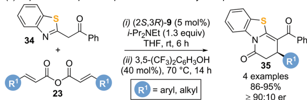
Scheme 10 Selective Michael–lactamization or Michael–lactonization using aryl esters.
