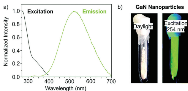
Fig. 20 (a) Emission spectrum at 274 nm and excitation spectrum at 274 nm of the synthesized GaN. (b) Photographs of the as synthesized GaN NCs in daylight and under excitation at 254 nm. Reprinted from ref. 168 with permission from the Royal Society of Chemistry.
