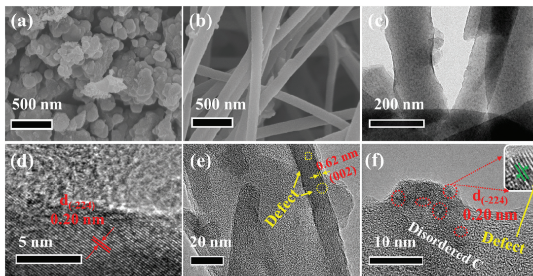
Fig. 1 SEM morphology of (a) P- \text{V}_5\text{S}_8/\text{C} and (b) D- \text{V}_5\text{S}_8/\text{CNFs} . (c) TEM image of D- \text{V}_5\text{S}_8/\text{CNFs} . The corresponding HRTEM images of (d) P- \text{V}_5\text{S}_8/\text{C} and (e and f) D- \text{V}_5\text{S}_8/\text{CNFs} . Note that the inset of (f) shows the relevant enlargement of the dashed box (red).
