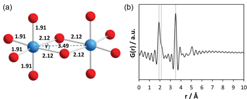
Fig. 2 (a) Model of the dimeric molecular structure of Ta 2 (OEt) 10 without the coordinating alcohol molecules as derived from EXAFS data and (b) the resulting calculated PDF. Blue and red spheres represent Ta and O atoms, respectively. The vertical dotted lines are a guide to the eye indicating the maxima of the peaks.
