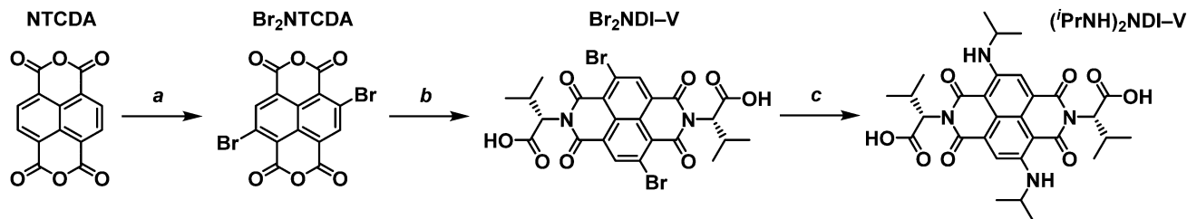
Scheme 2 The synthetic method to obtain core-functionalised blue ( i PrNH) 2 NDI-V. (a) Dibromoisocyanuric acid (2.5 eq.), H 2 SO 4 -20% SO 3 , 25 °C, 5 h, 29% yield. (b) L-Valine (2 eq.), glacial acetic acid, 120 °C, 18 h, 76% yield. (c) Isopropylamine, 25 °C, 10 days, 80% yield.
