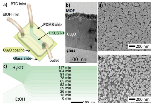
Fig. 3 (a) Schematic illustration of the in-flow MOF lithography method. (b) TEM cross-section image showing a densely-packed HKUST-1 film synthesized over a \text{Cu}_2\text{O} coated glass substrate. (c) Schematic representation of the time required to obtain compositionally graded HKUST-1 ( i.e. spatiotemporal controlled synthesis of a MOF film onto a surface). (d) and (e) SEM images of a graded HKUST-1 thin film. Note that the compactness of the HKUST-1 thin film varies throughout the width of the microchannel. Reproduced from ref. 41 with permission from Wiley-VCH Verlag GmbH & Co., copyright 2019.
