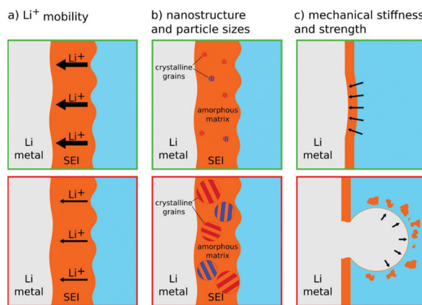
Fig. 5 Schematic illustration of how the SEI properties contribute to the lithium metal deposition morphology and how they can positively (top green boxes) or negatively (bottom red boxes) influence smooth electro-deposition. (a) High \text{Li}^+ mobility is desirable, (b) small crystalline grain size allows for more homogeneity, and (c) a stiff and strong SEI (high elastic modulus and high yield strength) can suppress whisker nucleation by pressing against lithium protrusions, while a SEI with low mechanical strength (low yield strength) breaks and allows whiskers to grow into the electrolyte.
