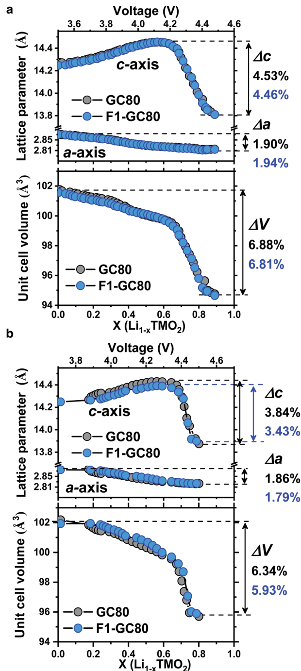
Fig. 5 Unit cell contraction of GC80 and F1-GC80 cathodes during delithiation. The lattice parameter and unit cell volume change for GC80 and F1-GC80 cathodes by in situ XRD analysis; (a) first cycle and (b) after 2000 cycles.
