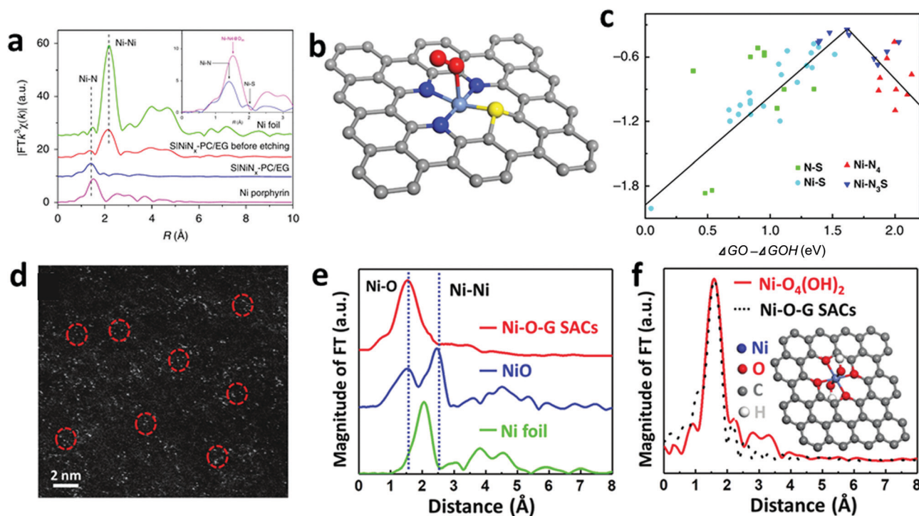
Fig. 18 (a) Fourier-transformed magnitudes of the experimental K-edge EXAFS signals of Ni-N 3 S SAC. (b) Structural geometry of Ni-N 3 S SAC with O-S. (c) OER volcano plot of the overpotential \eta vs. the difference between the adsorption free energy of \text{*O} and \text{*OH} for the N-S, Ni-S, Ni-N 4 , and Ni-N 3 S models. Reproduced with permission from ref. 353. Copyright 2019, Springer Nature. (d) Atomic-scale HAADF-STEM image of Ni-O 4 -G SACs. (e) FT-EXAFS spectra of Ni-O 4 -G SACs with NiO and Ni foil references. (f) FT-EXAFS data of the proposed Ni-O 4 (OH) 2 architecture compared to experimental Ni-O 4 . Reproduced with permission from ref. 354. Copyright 2020, Wiley VCH.
