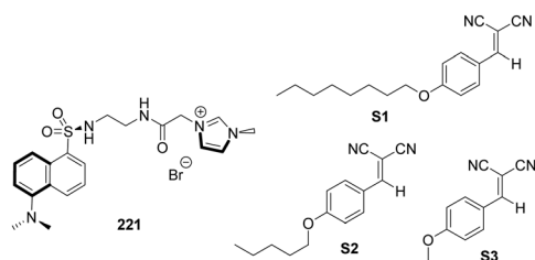
Fig. 34 Structures of imidazolium-bearing dansyl-based probe 221 and the benzyldenemalononitrile substrates ( S1 , S2 and S3 ).
