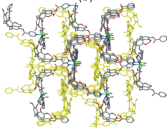
Fig. 14 Examples of other coordination polymers with different types of guest-accessible spaces. (a) [\text{Ag}_2(\text{L}2)(\text{DMF})_2] \cdot 2(\text{BF}_4) \cdot 2(\text{H}_2\text{O}) packing with guests shown in space-fill; 21 (b) two stacked networks of [\text{Cu}_5(\text{L}19)_2\text{Cl}_{10}(\text{NMP})_4] \cdot n(\text{NMP}) with intracavity NMP in space-fill, coordinated NMP in purple and lattice NMP in pale pink; 17 (c) [\text{Cu}_2(\text{L}1)_2(\text{NMP})(\text{H}_2\text{O})] \cdot 4(\text{BF}_4) \cdot 12(\text{NMP}) \cdot 1.5(\text{H}_2\text{O}) with one of two interpenetrating networks in yellow and all guest solvent and anions not shown. 20
