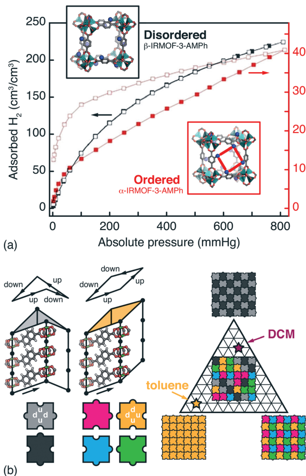
Fig. 4 Orientational disorder in MOFs. (a) The \alpha - and \beta -polymorphs of the substituted MOF-5 derivative IRMOF-3-AMPh have different linker orientation correlations and \text{H}_2 (de)adsorption profiles. Using the fully substituted AMPH-terephthalate linker during MOF synthesis gives the ordered \alpha phase, with reduced and hysteretic \text{H}_2 uptake is sorption profile. By contrast, post-synthetic modification of an aminoterephthalate MOF-5 derivative gives the disordered \beta phase, which has a greater accessible pore volume. 71 Adapted from ref. 71 with permission from the Royal Society of Chemistry. (b) In the pillared MOF DUT-8(Ni), naphthalenedicarboxylate linkers introduce a 'step-up'/'step-down' between neighbouring columns (exaggerated for effect here). There are six feasible NDC arrangements— i.e. two steps up and two steps down—around the lozenge-shaped pores. These arrangements give pores with either D_{2d} or C_{2v} point symmetry (grayscale and coloured tiles, respectively) that propagate according to a set of simple rules (jigsaw pairings shown here). Different guest molecules have different affinities for these two pore geometries, which allows a guest-induced transition between complex phases; for example, toluene and dichloromethane (DCM) favour configurations with C_{2v} - and D_{2d} -rich pore geometries, respectively. 15
