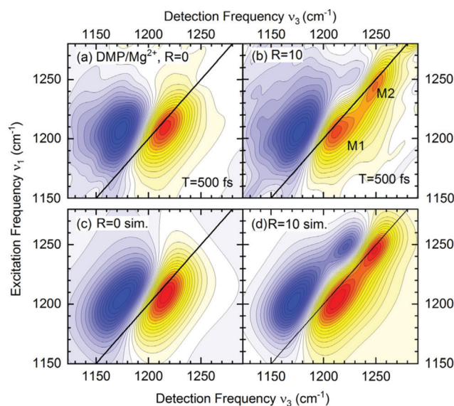
Fig. 7 (a and b) 2D-IR spectra of DMP \nu_3 in water in the range of the \nu_{\text{AS}}(\text{PO}_2)^- vibrations for a waiting time T = 500\text{ fs} . The absorptive 2D signal is shown as a function of the excitation frequency \nu_1 and the detection frequency \nu_3 : yellow-red contours represent signals due to the fundamental ( \nu = 0-1 ) transition, and blue contours the excited state \nu = 1-2 absorption. Signal changes between neighbouring contour lines are 7.5%. R = c(\text{Mg}^{2+})/c(\text{DMP}) is the ratio of \text{Mg}^{2+} to DMP concentration. (c and d) Simulated 2D-IR spectra for R = 0 and R = 10 . Adapted with permission from ref. 75. Copyright 2021 American Chemical Society.
