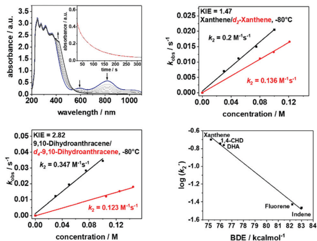
Fig. 3 Top left: Changes in the UV-Vis-spectra of a 1 mM solution of 1-trans in \text{CH}_2\text{Cl}_2/\text{CH}_3\text{CN} (95:5) at -80\text{ }^\circ\text{C} upon addition of 100 eq xanthene; the inset shows the time trace for the decay of the 815 nm band and its pseudo-first order fit; top right: plots of the pseudo-first order rate constants k_{\text{obs}} vs. the substrate concentrations for xanthene and d_2 -xanthene in order to determine the kinetic isotopic effect (KIE) for the reaction of 1-trans with xanthene; bottom left: plots of the pseudo-first order rate constants k_{\text{obs}} vs. the substrate concentrations for 9,10-dihydroanthracene (DHA) and d_4 -DHA in order to determine the kinetic isotopic effect (KIE) for the reaction of 1-trans with DHA; bottom right: plot of the logarithms of the second-order rate constants k_2' vs. the C-H BDEs of the substrates with 1-trans in \text{CH}_2\text{Cl}_2/\text{CH}_3\text{CN} (95:5).
