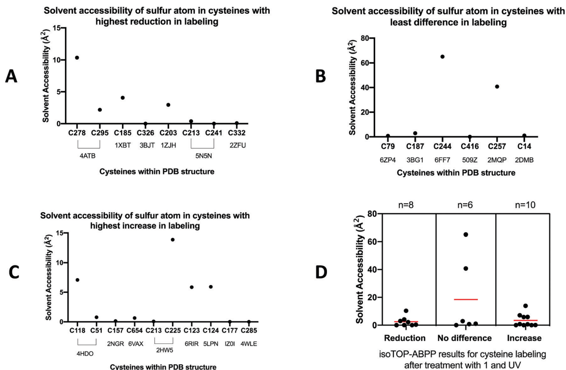
Fig. 10 Solvent accessible surface area of sulphur atoms in cysteines with highest reduction in labeling of peptides with resolved crystal structures.
