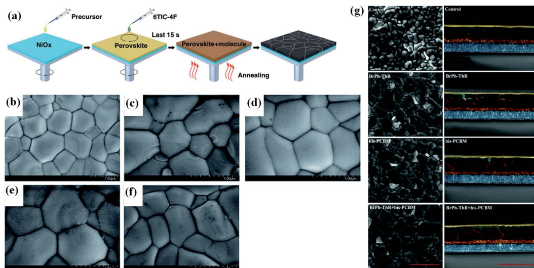
Fig. 8 (a) Schematic diagram of the deposition processes of the prepared CsPbBr_{x-1}I_x perovskite film. Reproduced by the permission of ref. 82, Copyright 2020, Springer Nature. Top-view scanning electron microscope images of (b) CsPbBr_3 , (c) CsPb_{0.97}Mg_{0.03}Br_3 , (d) CsPb_{0.97}Ca_{0.03}Br_3 , (e) CsPb_{0.97}Sr_{0.03}Br_3 and (f) CsPb_{0.96}Ba_{0.04}Br_3 films. Reproduced by permission ref. 84, Copyright 2019 Royal Society of Chemistry. (g) SEM images. Top (left, the scale is 1 mm) SEM of corresponding perovskite films and cross-sectional (right, the scale is 2 mm) SEM of corresponding perovskite devices. (1) Control; (2) BrPh-ThR; (3) bis-PCBM; and (4) BrPh-ThR + bis-PCBM. Reproduced by permission ref. 85, Copyright 2018 Royal Society of Chemistry.
