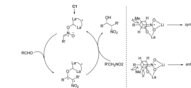
Scheme 2 The mechanism of C1 catalyzed asymmetric Henry reaction.
