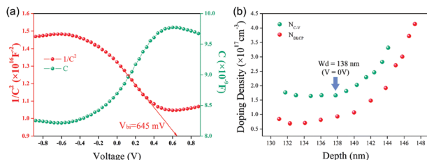
Fig. 12 (a) The C-V (green) and 1/C^2 - V (red) curves for the GeSe solar cell tested at room temperature under dark conditions. (b) C-V profiling and DLCP profiling for the GeSe solar cell. Reprinted with permission from ref. 56. Copyright 2019, Royal Society of Chemistry.
